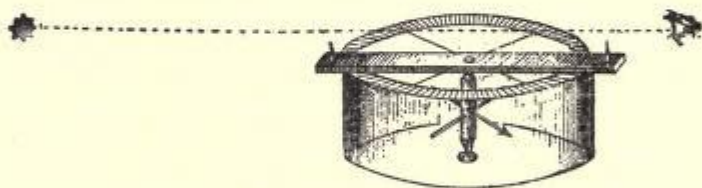
FIG. 3.—PIVOTED COMPASS
